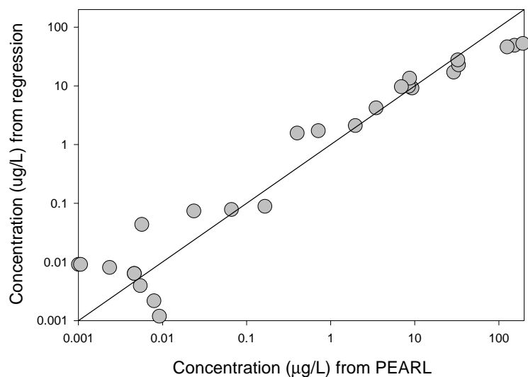
Figure 2. Comparison of leaching concentrations as calculated with PEARL with leaching concentrations calculated with Equation 40. The points are concentrations and the line is the 1:1 line.
