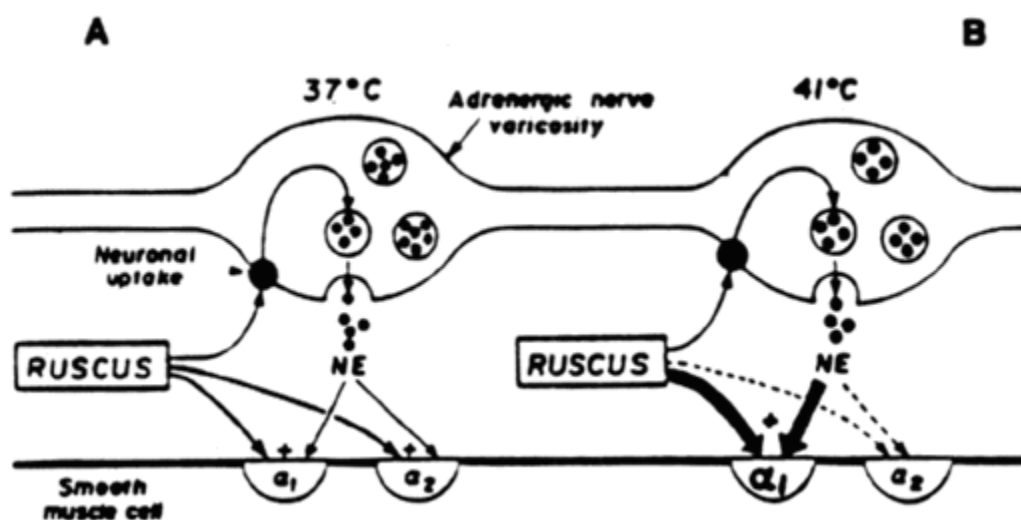
Figure 1: Proposed mechanism of action for Ruscus and effect of temperature (Marcelon and Vanhoutte, 1988)
