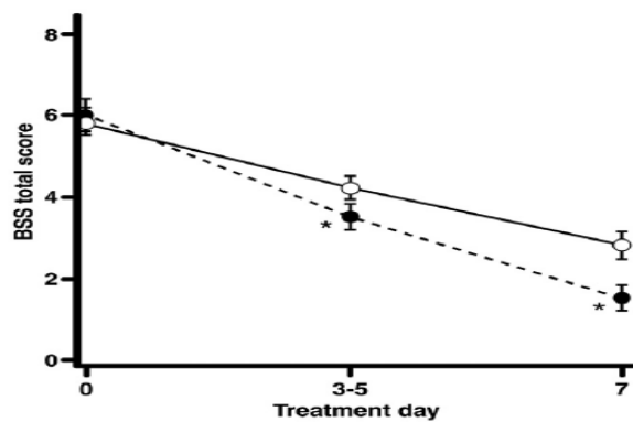
Fig. 3 Time-course of the bronchitis-specific symptoms (BSS) total score (mean, 95% confidence interval). ( \circ ) Placebo; ( \bullet ) EPs 7630 (* p < 0.0001 ; ANCOVA)
