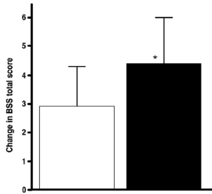
Figure 32: Change in bronchitis-specific symptoms (BSS) total score (mean \pm SD) ( \square ) Placebo; ( \bullet ) EPs 7630 (* p < 0.0001 , ANCOVA) (Kamin et al. , 2012)
