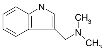
Figure 1: the alkaloid gramine
